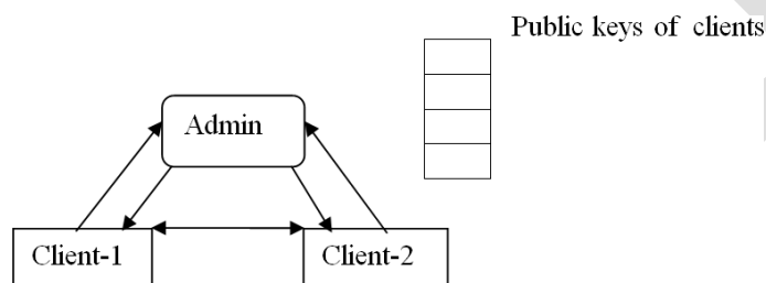
Figure 2: Secure Communication
